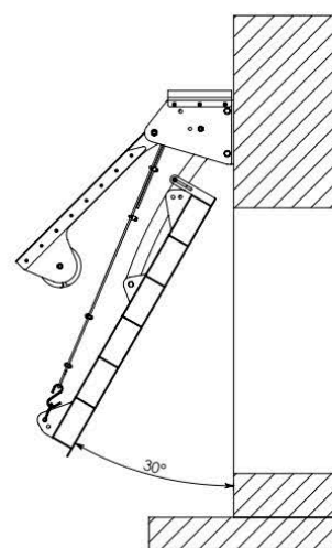
Flap Fully Open - 30° Scale 1 : 20
