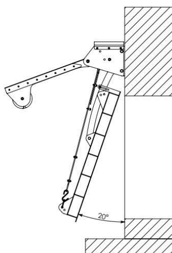
Flap 20° Open Scale 1 : 20
