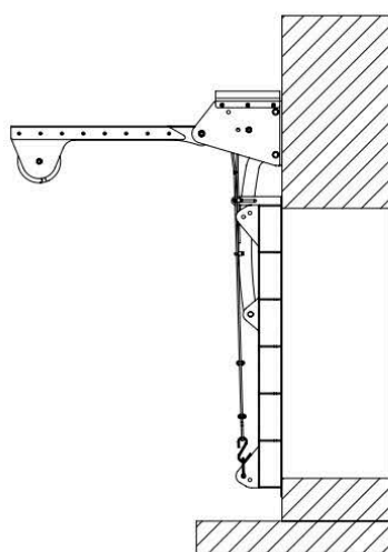
Flap Closed Scale 1 : 20
