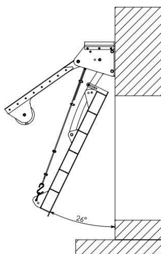
Flap 26° Open Scale 1 : 20
