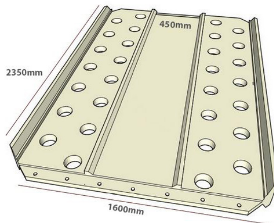
Floating Wetland unit shown with standard dimensions and modular planting cell layout.
